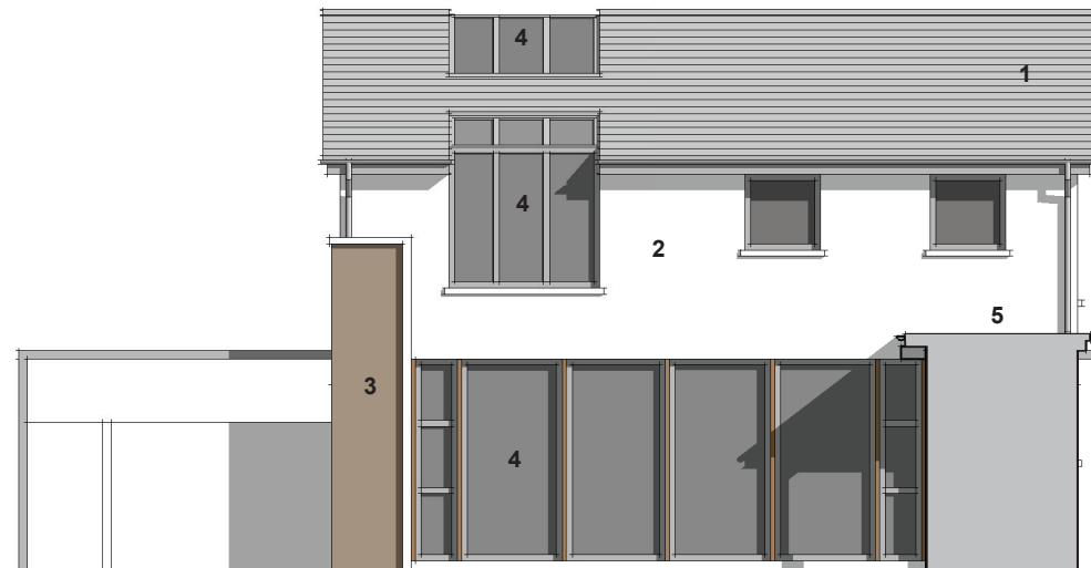
PROPOSED ELEVATION - ELE 5
