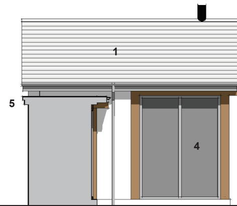
PROPOSED ELEVATION - ELE 7
