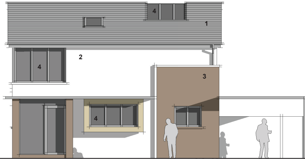
PROPOSED FRONT ELEVATION - ELE 1
