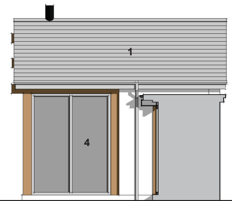
PROPOSED ELEVATION - ELE 8
